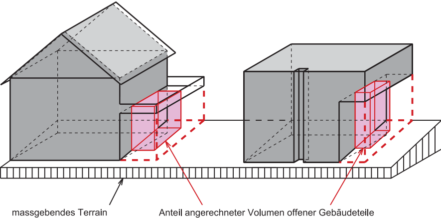
Figur 8.3 Baumassenziffer
